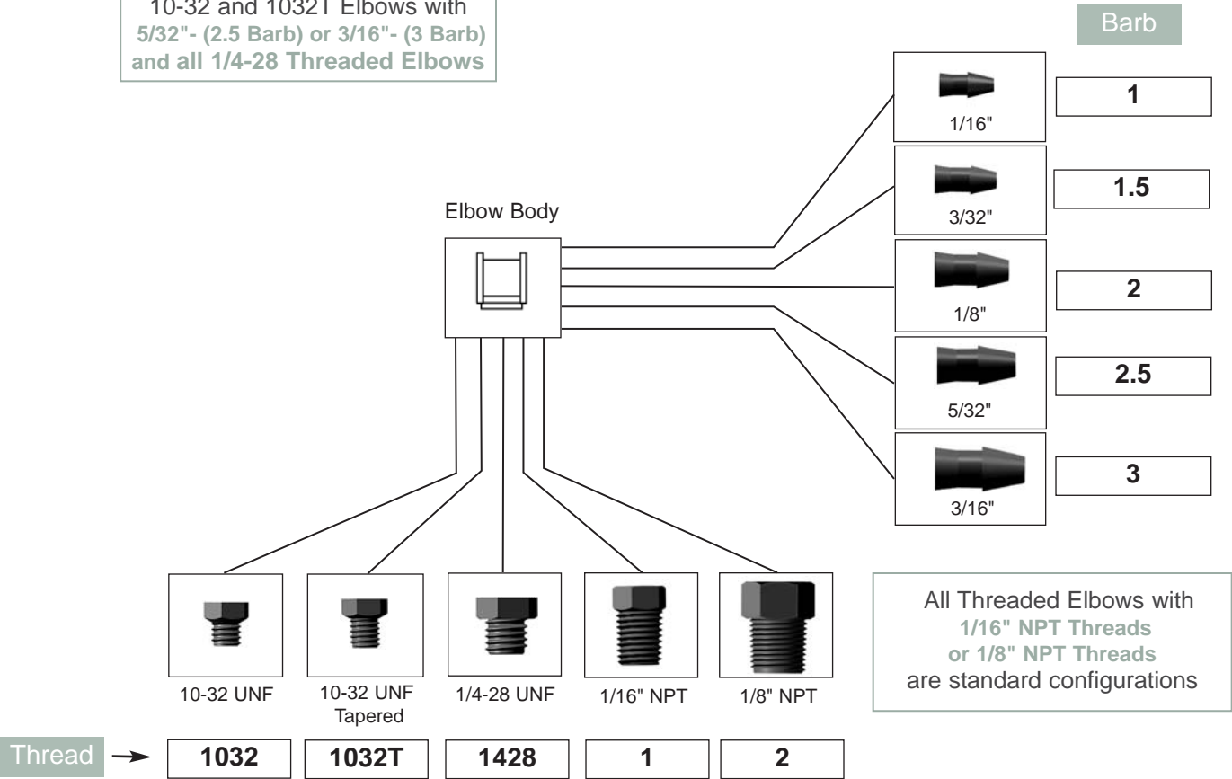
Threaded Elbow
