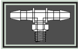
Threaded Tee - Equal Barbs
