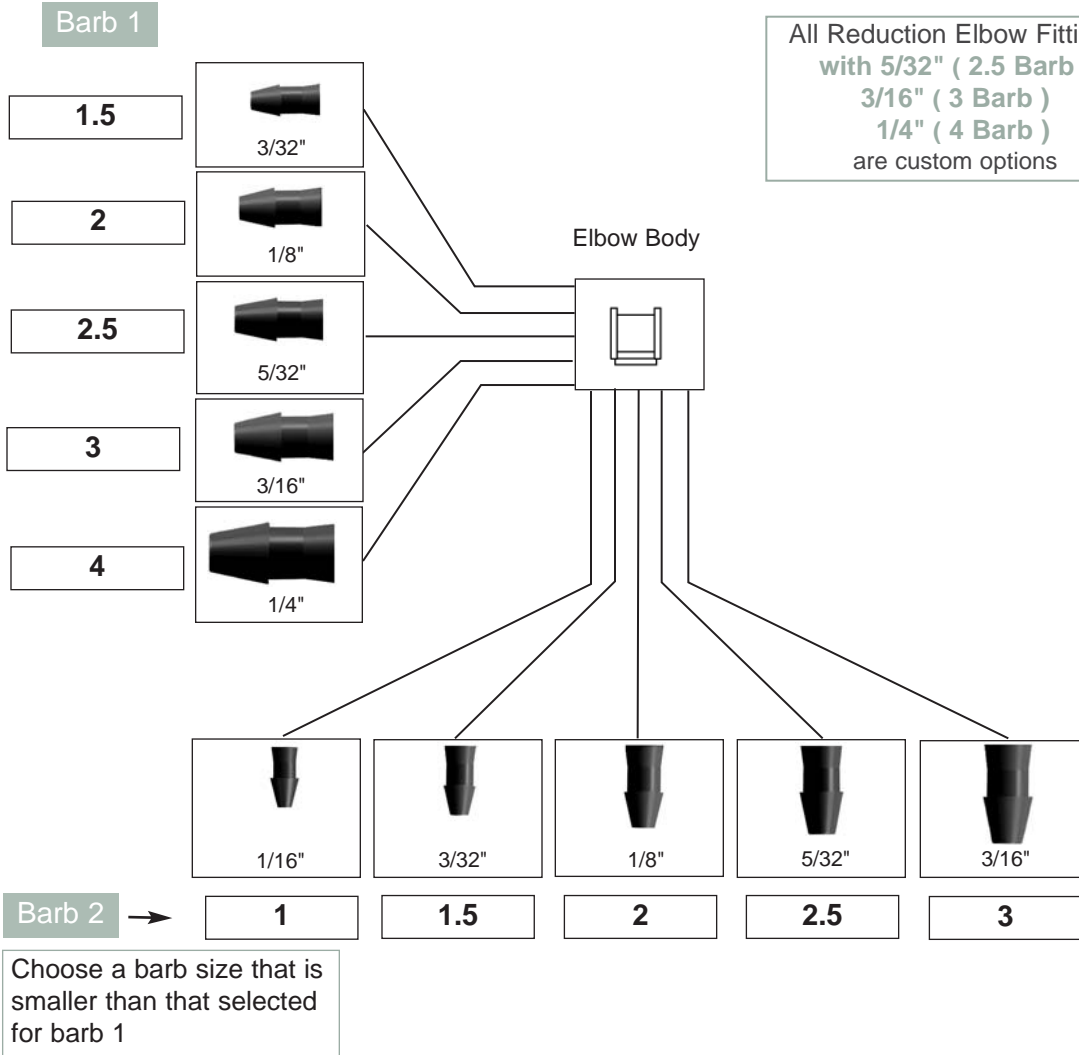
Barbed Reduction Elbow
